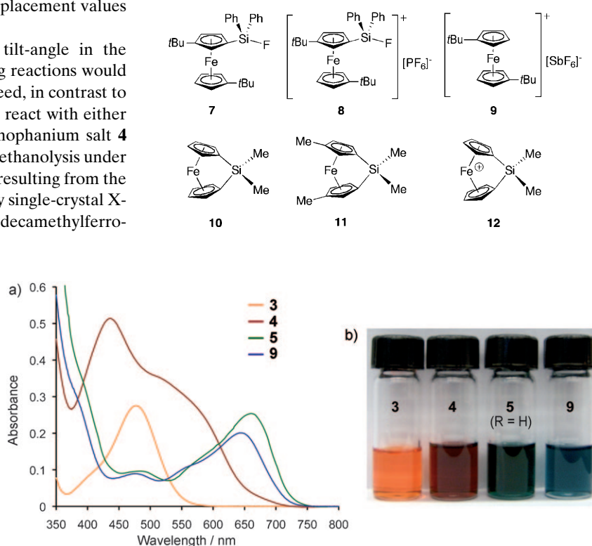
Figure 2. a) UV/Vis spectra of 3 , 4 , 5 (R = H), and 9 . b) Photographs of these species in CH 2 Cl 2 solutions.
